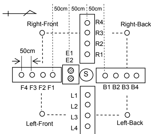
Fig. 1 Arrangement of Data Collection Points F: front, B: back, R: right, L: Left
